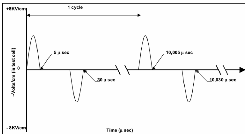
Figure 3. Pulsed wave form at 100 and 200 Hz (two cycles at 100 hz depicted) for the electric field study conducted in 2000
